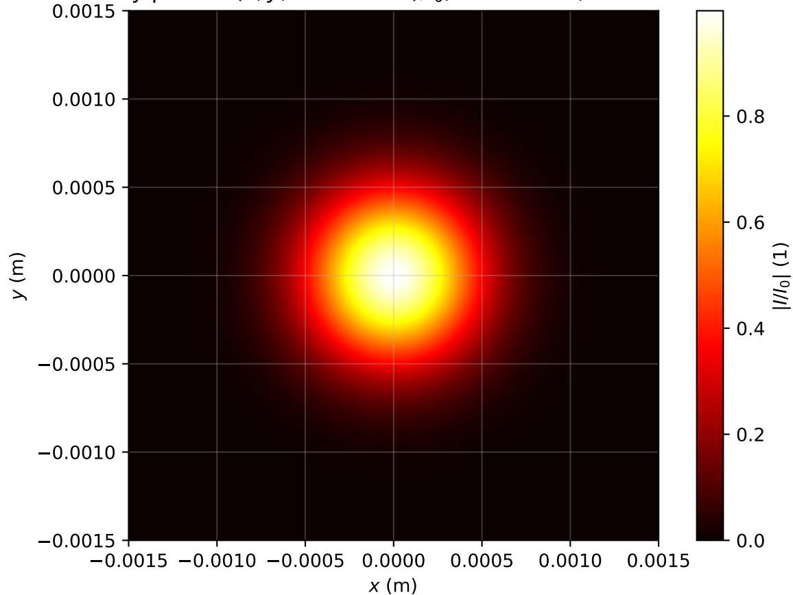
Intensity profile I(x, y, z = 0.159m)/I_0 , Pin=0.2Pcr, artificial time
